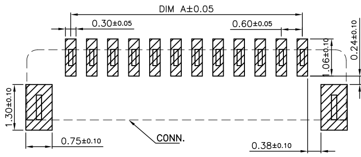
P. C. B Layout
